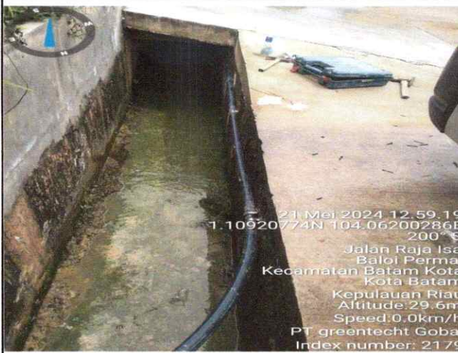
PASANG KLEM HDPE
